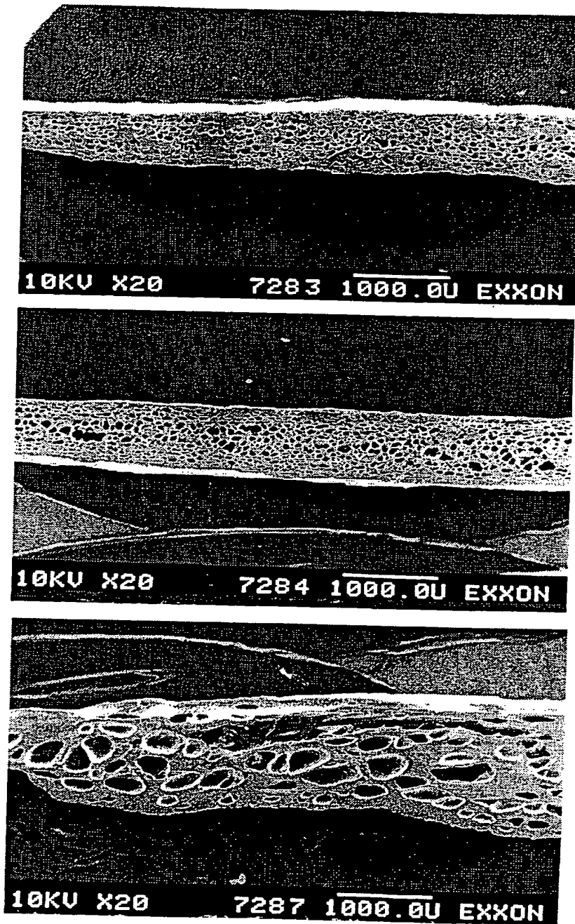
Figure 9: Morphologies of flat foamed sheets from Examples 10, 7 and commercial product PF-814 (chemical blowing agent)
